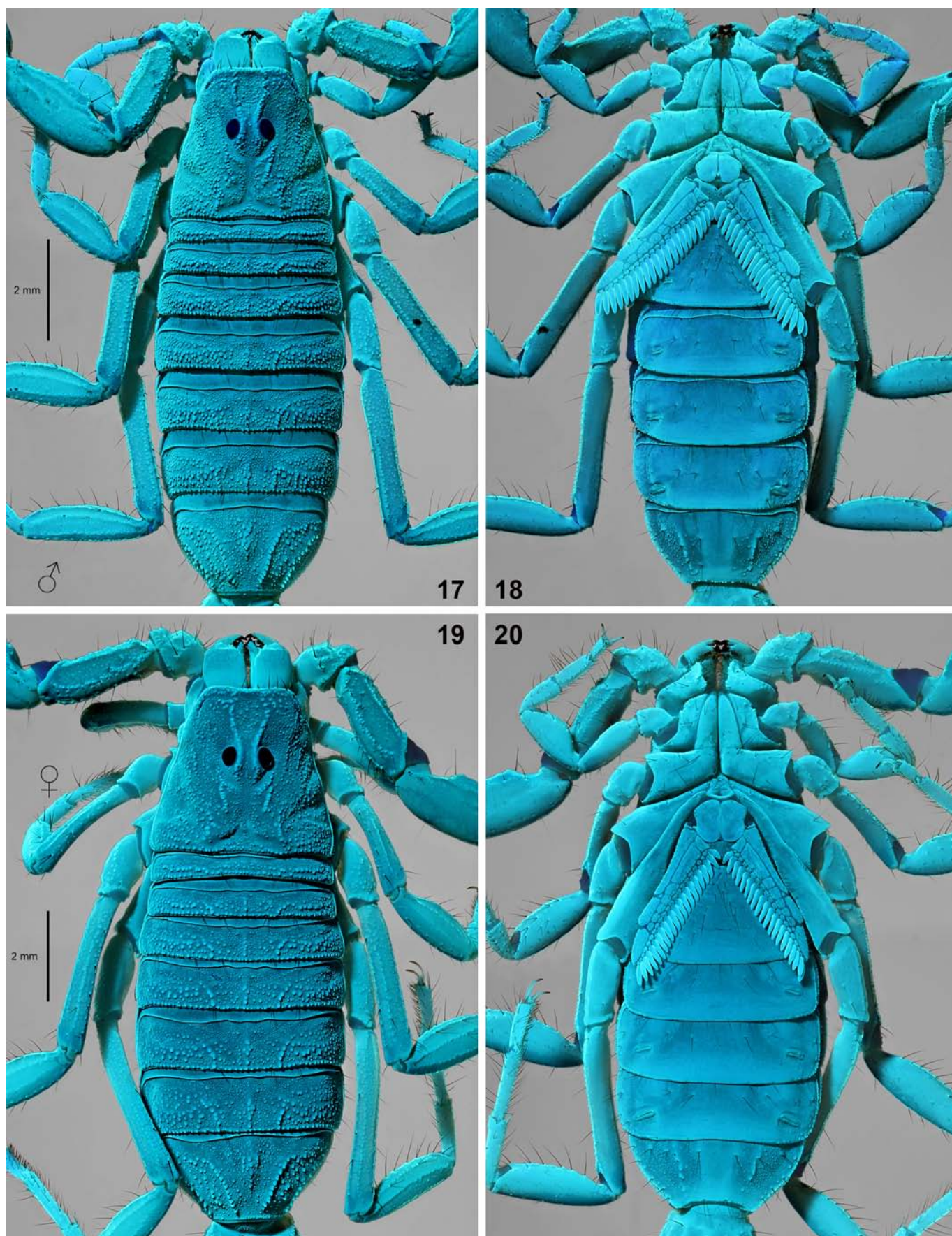
Figures 17–20: Somalibuthus sabae sp. n., carapace and tergites (17, 19) and coxosternal area and sternites (18, 20), under UV fluorescence. Figures 17–18. Paratype male. Figures 19–20. Paratype female. Scale bar: 2 mm (17–18, 19–20).
