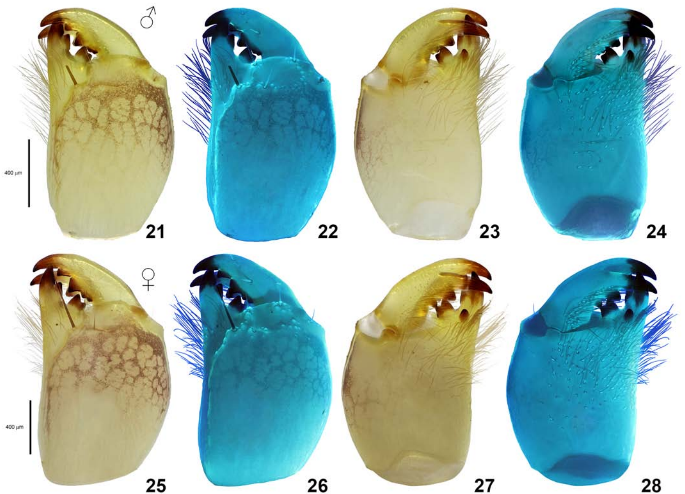
Figures 21–28: Somalibuthus sabae sp. n., chelicerae. Figures 21–24. Paratype male, right chelicera in dorsal (21–22) and ventral (23–24) views, under white light (21, 23) and UV fluorescence (22, 24). Figures 25–28. Paratype female, right chelicera in dorsal (25–26) and ventral (27–28) views, under white light (25, 27) and UV fluorescence (26, 28). Scale bars: 400 µm (21–24, 25–28).
