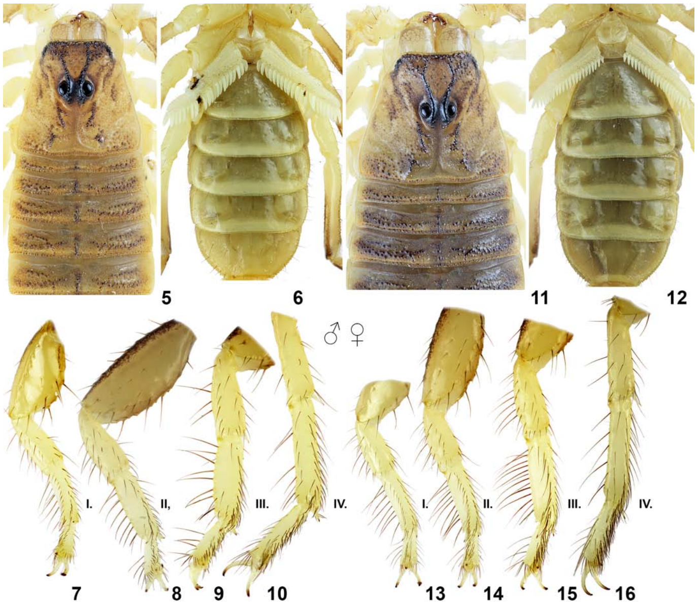
Figures 5–16: Somalibuthus sabae sp. n. Figures 5–10. Holotype male. Carapace and tergites I–V (5), sternopectinal area and sternites (6), and left legs I–IV, retrolateral aspect (7–10). Figures 11–16. Paratype female. Carapace and tergites I–IV (11), sternopectinal area and sternites (12), and left legs I–IV, retrolateral aspect (13–16).
