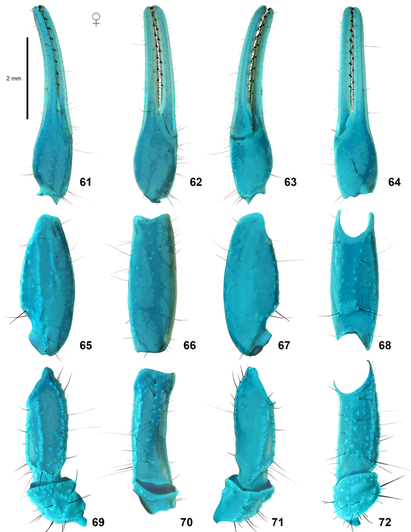
Figures 61–72: Somalibuthus sabae sp. n., paratype female, right pedipalp under UV fluorescence. Figures 61–64. Chela in dorsal (61), external (62), ventral (63) and internal (64) views. Figures 65–68. Patella in dorsal (65), external (66), ventral (67) and internal (68) views. Figures 69–72. Femur and trochanter in dorsal (69), external (70), ventral (71) and internal (72) views. Scale bar: 2 mm.
