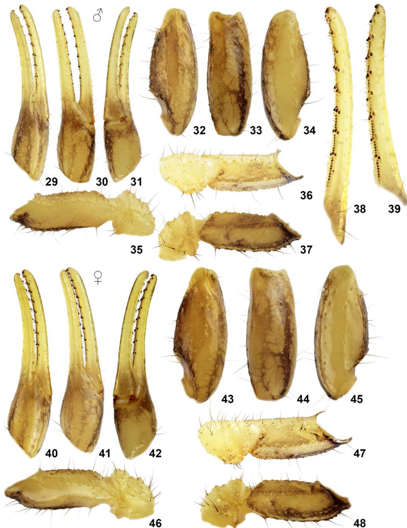
Figures 29–48: Somalibuthus sabae sp. n., right pedipalp under white light. Figures 29–39. Holotype male, chela in dorsal (29), external (30) and ventral (31) views, patella in dorsal (32), external (33) and ventral (34) views, femur in ventral (35), internal (36) and dorsal (37) views, dentate margins of movable finger (38) and fixed finger (39). Figures 40–48. Paratype female, chela in dorsal (40), external (41) and ventral (42) views, patella in dorsal (43), external (44) and ventral (45) views, femur in ventral (46), internal (47) and dorsal (48) views.
