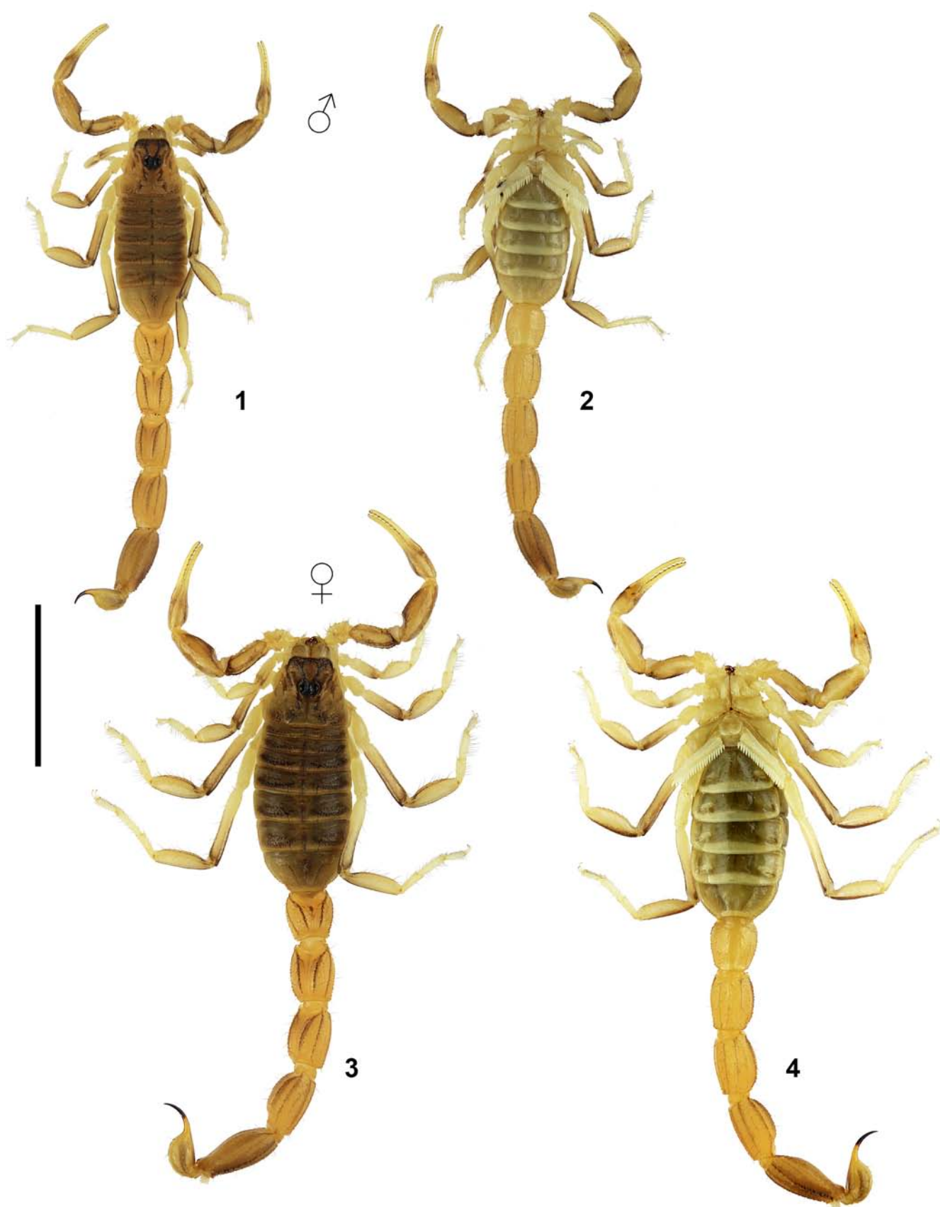
Figures 1–4: Somalibuthus sabae sp. n., habitus. Figures 1–2. Male holotype in dorsal (1) and ventral (2) views. Figures 3–4. Female paratype in dorsal (3) and ventral (4) views. Scale bar: 10 mm.
