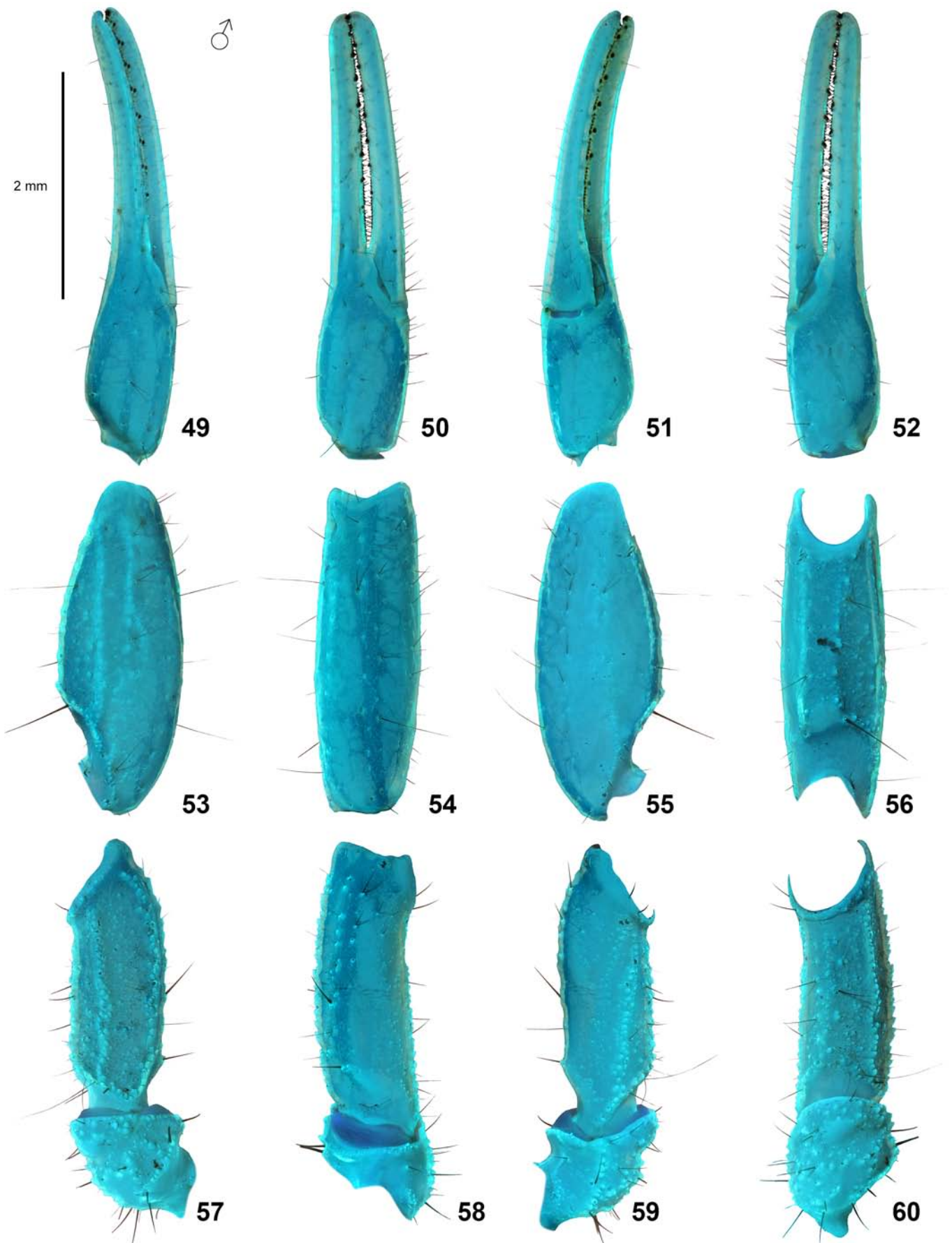
Figures 49–60: Somalibuthus sabae sp. n., paratype male, right pedipalp under UV fluorescence. Figures 49–52. Chela in dorsal (49), external (50), ventral (51) and internal (52) views. Figures 53–56. Patella in dorsal (53), external (54), ventral (55) and internal (56) views. Figures 57–60. Femur and trochanter in dorsal (57), external (58), ventral (59) and internal (60) views. Scale bar: 2 mm.
