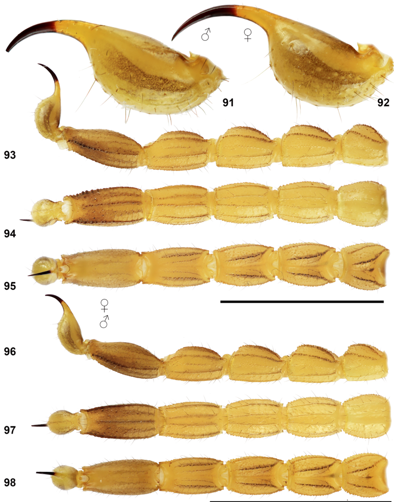
Figures 91–98: Somalibuthus sabae sp. n., metasoma and telson under white light. Figures 91–92. Telson in right lateral view of holotype male (91) and paratype female (92). Figures 93–95. Paratype female, metasoma and telson in right lateral (93), ventral (94) and dorsal (95) views. Figures 96–98. Holotype male, metasoma and telson in right lateral (96), ventral (97) and dorsal (98) views. Scale bars: 10 mm (93–95), 10 mm (96–98).
