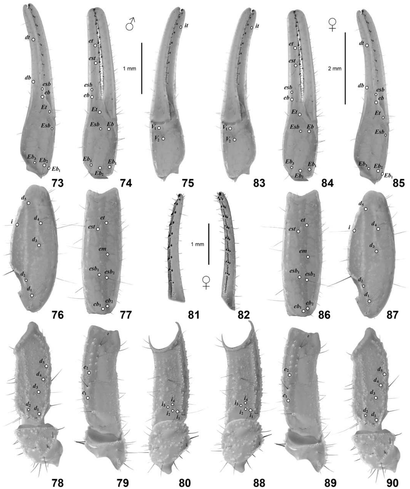
Figures 73–90: Somalibuthus sabae sp. n., right pedipalp, trichobothrial maps and finger dentition. Figures 73–80: Paratype male trichobothria, chela in dorsal (73), external (74) and ventral (75) views, patella in dorsal (76) and external (77) views, femur in dorsal (78), external (79) and internal (80) views. Figures 81–82: Paratype female dentition of fixed (81) and movable (82) fingers. Figures 83–90: Paratype female trichobothria, chela in ventral (83), external (84) and dorsal (85) views, patella in external (86) and dorsal (87) views, femur in internal (88), external (89) and dorsal (90) views. Scale bars: 1 mm (73–80), 1 mm (81–82), 2 mm (83–90).
